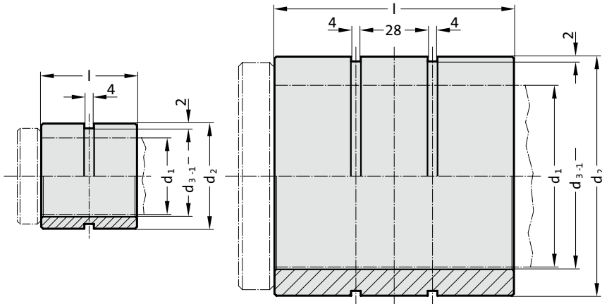
Mounting example
