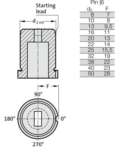
Anti-rotation element 3 (3)
