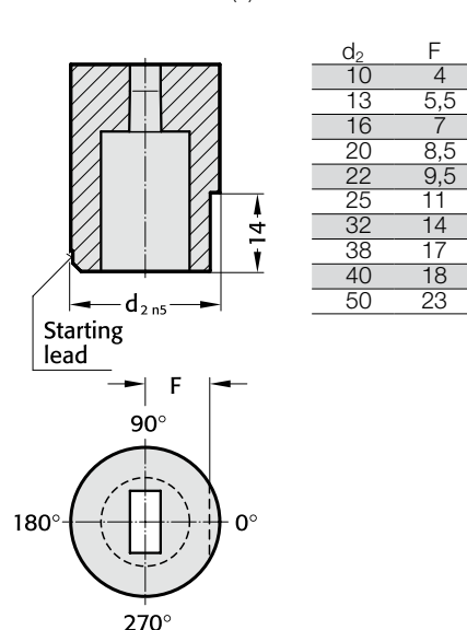
Anti-rotation element 6 (6)
