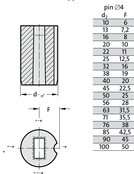
Anti-rotation element 2 (2)
