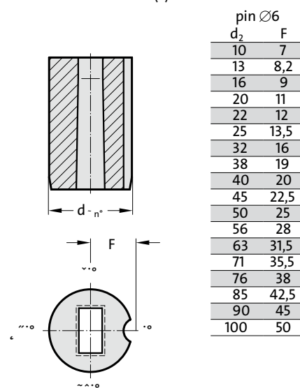
Anti-rotation element 3 (3)
