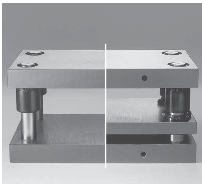
without Stripper
