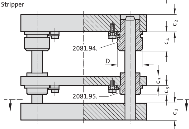
with Stripper
