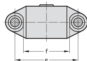
Section A - A
