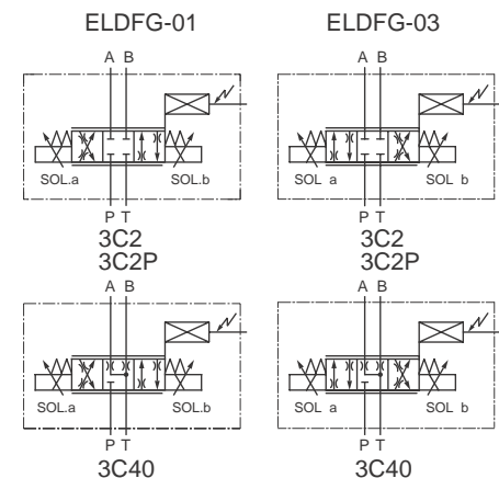
Graphic Symbols
