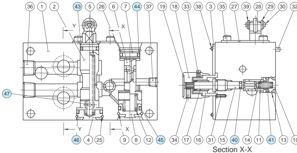
Section X-X
