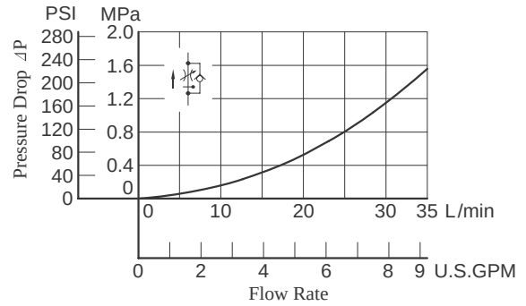
Pressure Drop at Throttle Fully Open
