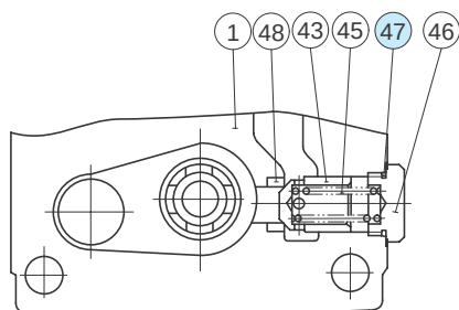
Section X-X (FCG-10 Type)
