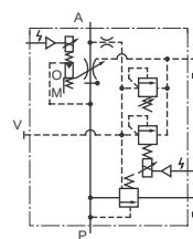
Models with Proportional Pilot Relief Valve
