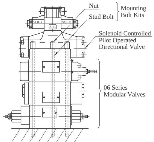
Stacking Example
