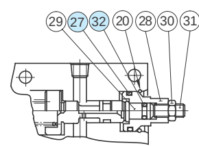
Section X-X (FG/FCG-01-*-N Type)
