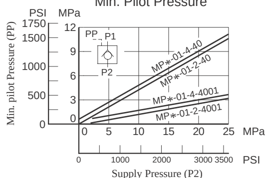
Min. Pilot Pressure
