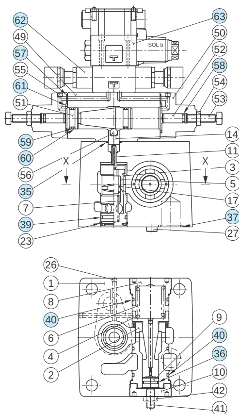
(FHG-* Type) Section X-X
