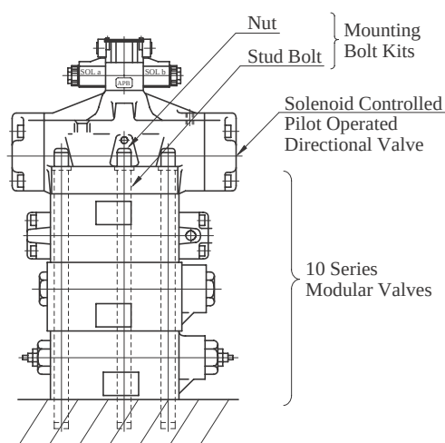
Stacking Example
