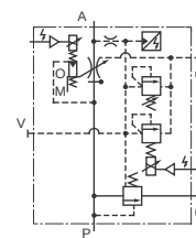
Models with Proportional Pilot Relief Valve and Sensor
