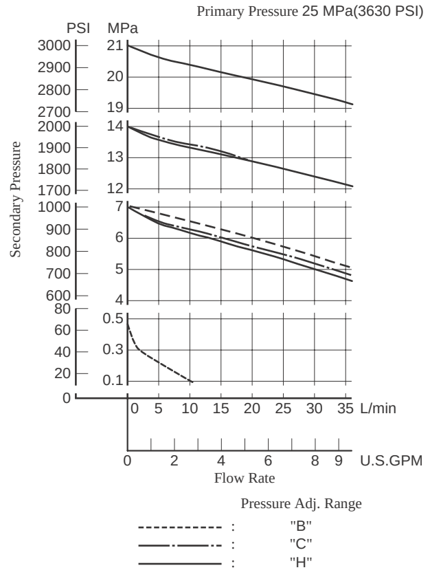
Nominal Override Characteristics
